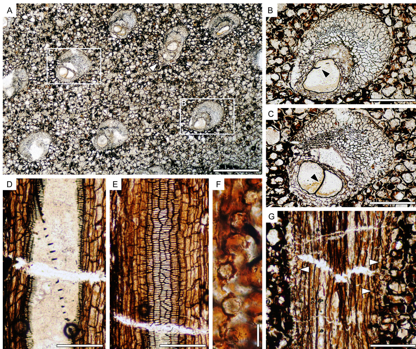
FIGURE 2 Palmoxydon sp.1 (Arecaceae). (A–C) MNHN.F.50226.1, transverse sections; (D–G) MNHN.F.50226.3, tangential longitudinal sections. (A) Arrangement of fibrous-vascular bundles (fvb) in a mostly spheroid-compact ground parenchyma with some small lacunae and the beginning of a leaf trace (arrowhead). Boxes outline the area detailed in B and C. (B, C) A fvb with reniforma fibrous dorsal cap. Phloem cells are missing, the perivascular parenchyma is developed. Mostly one vessel element is present in each fvb (arrowheads: bars of scalariform perforations). (D) “Oblique” scalariform perforation with 20 bars on average, surrounded by perivascular parenchyma. (E) Perivascular parenchyma and vessel-parenchyma pits. (F) Globular echinate phytoliths. (G) Globular echinate phytoliths (arrowheads) surrounding the fibers of a fibrous dorsal cap, spheroid (to slightly elongated cells) and compact ground parenchyma on each side. Scale bars: (A) 1 mm; (B–E, G) 200 \mu m ; (F) 25 \mu m .
