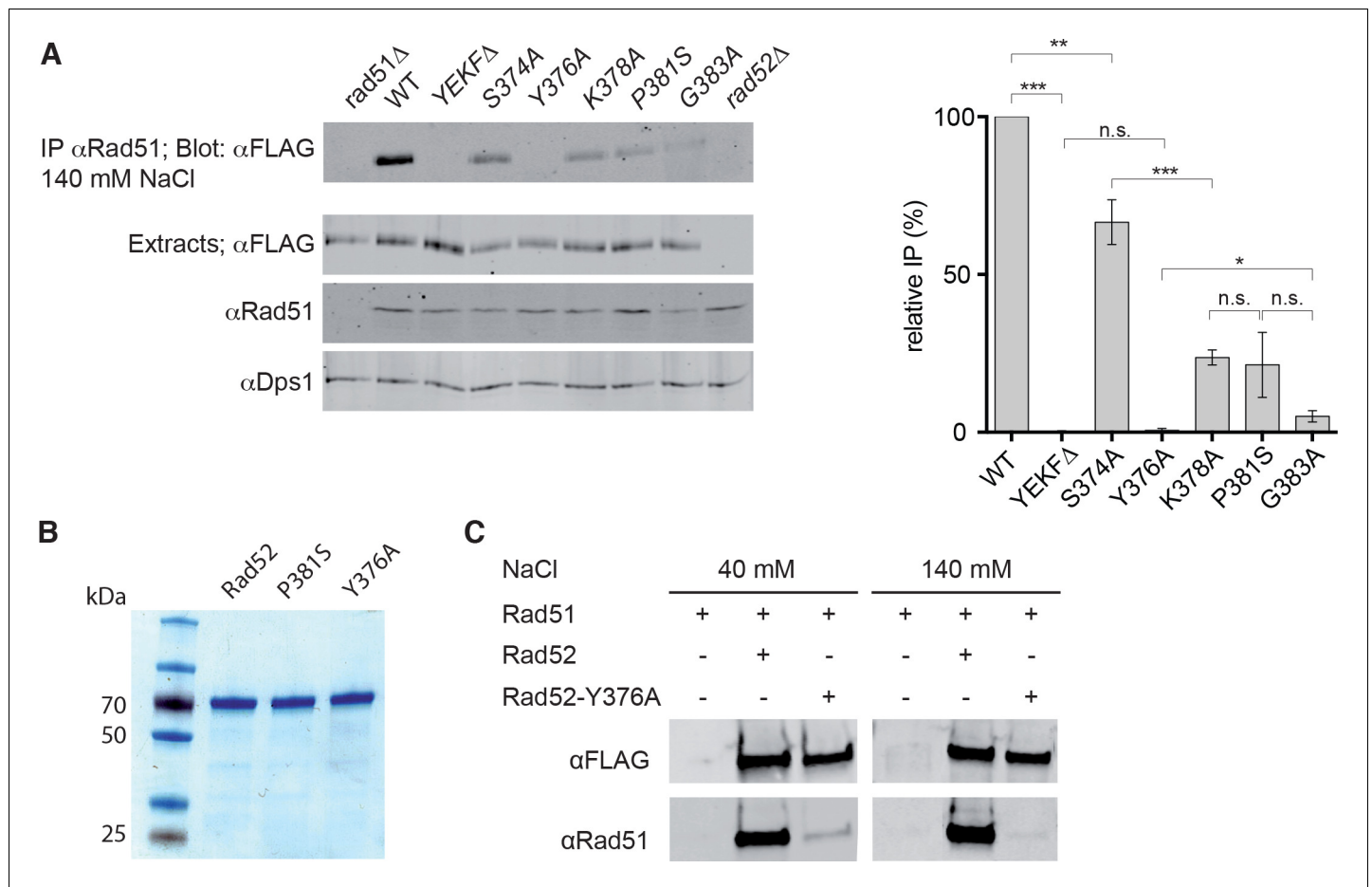
Figure 2. Measurement of Rad52-Rad51 interaction in cells that express various Rad52-FLAG mutants. (A) Rad51 immunoprecipitation from cells that express different Rad52-FLAG mutants. The anti-Dps1 antibody was used as loading control. The signals corresponding to immunoprecipitated Rad52 mutants (Blot: \alpha FLAG) were quantified relatively to the signal for WT Rad52, corrected to the quantity of Rad52 in each extracts (Extracts: \alpha FLAG) and to the Dps1 signal ( \alpha Dps1). Data are presented as the mean \pm SEM ( n = 3 ). Fisher's exact test, n.s. p > 0.05 , * p < 0.05 , ** p < 0.01 , *** p < 0.001 . (B) Purification of recombinant Rad52-FLAG, Rad52-P381S-FLAG and Rad52-Y376A-FLAG. (C) Pull-down experiments using Rad52-FLAG WT or Y376A fusion protein in the presence of different salt concentrations.
