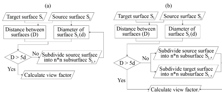
Figure 3. (a) Flowchart of optimized ISA method. (b) Flowchart of optimized Nusselt method.
