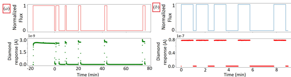
Figure 5 Response of the 550 μm diamond during 160 kV X-ray tube irradiation (a), and 95 keV monochromatic synchrotron radiation (b). During both irradiations the irradiated area was 0.5 \text{ mm} \times 0.5 \text{ mm} .
