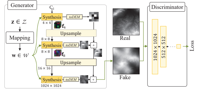
Figure 3: StyleGAN2 architecture. A vector from the latent space \mathcal{Z} is projected into a second latent space \mathcal{W} \in \mathcal{W} by using a mapping network that disentangles latent directions. \mathbf{w} is then streamed to the generator at various levels of resolution, and the output is sent to a discriminator, which seeks to separate real and fake images. The generator and the discriminator are trained together in a zero-sum game. The results are utilised during the backward generation phase. The toDEM component corresponds to the toRGB layer in the original StyleGAN2 which has been modified to handle a single channel image.
