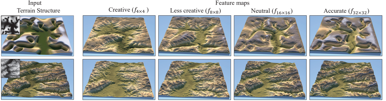
Figure 9: Influence of the feature maps insertion at the i -th level: the user can adjust the creativity or prefer adherence to the input. If they prefers reproducing the terrain as accurately as possible, they can employ the fourth level. In contrast, if they wants to draw a draft, they may use a low-level feature map.
