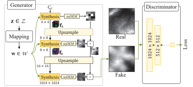
Figure 3: StyleGAN2 architecture. A vector from the latent space \mathcal{Z} is projected into a second latent space \mathbf{w} \in \mathcal{W} by using a mapping network that disentangles latent directions. \mathbf{w} is then streamed to the generator at various levels of resolution, and the output is sent to a discriminator, which seeks to separate real and fake images. The generator and the discriminator are trained together in a zero-sum game. The results are utilised during the backward generation phase. The toDEM component corresponds to the toRGB layer in the original StyleGAN2 which has been modified to handle a single channel image.
