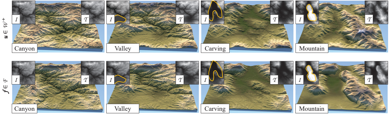
Figure 20: An ablation study on the importance of the features maps: when using feature maps (bottom), large structures of the terrain are faithfully reconstructed while keeping details where the user edited using a mask and a combination of multiple levels of features maps.
