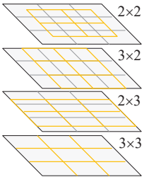
Figure 10: Patch decomposition.
