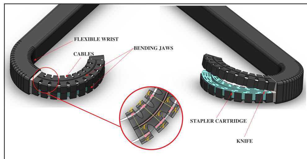
Figure 9. FLEXible surgical stapler design
