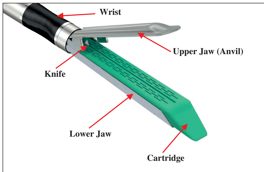
Figure 1. Various parts of a conventional endoscopic surgical stapler.
