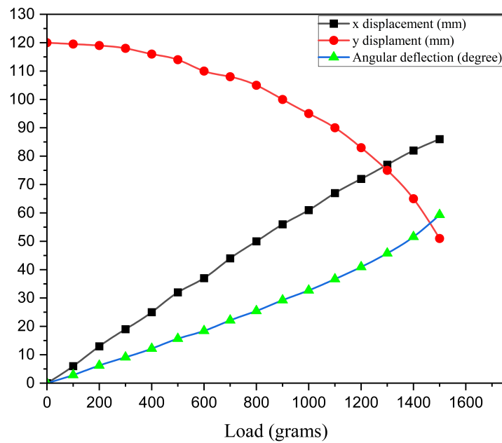
Figure 12. Plot of x displacement, y displacement and angular deflection of prototype tip ( \alpha ) vs. load applied, as presented in Table 2.
