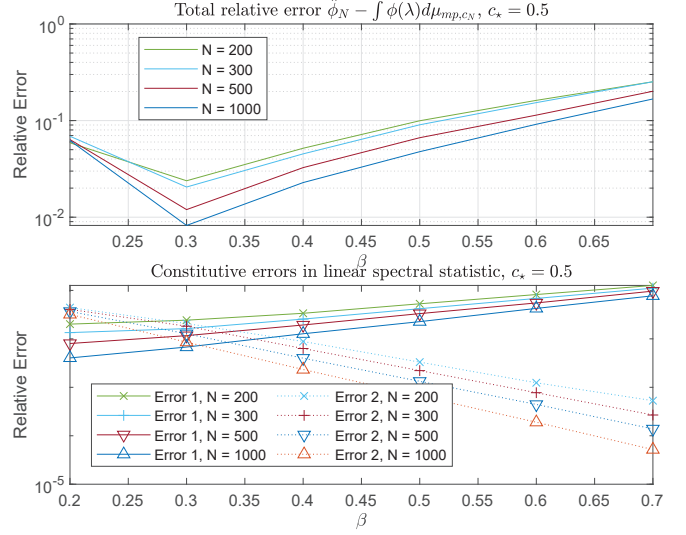
Fig. 2. Evolution of the error of \hat{\phi}_N with respect to the Marchenko-Pastur limit as a function of \beta .
