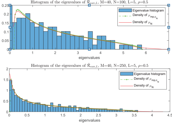
Fig. 1. Histogram of the eigenvalues of \widehat{\mathcal{R}}_{\text{corr},L} in comparison with the distributions \mu_N and \mu_{mp,c_N} for different values of M, N, L with \rho = 0.5 . The upper plot corresponds to a situation where c_N > 1 whereas the lower plot represents the case c_N < 1 .
