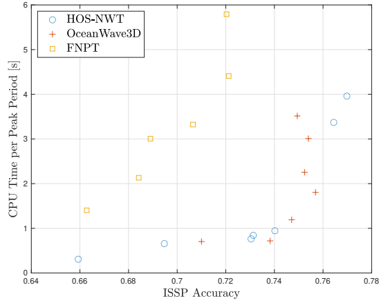
Figure 40: CPU time versus ISSP accuracy for the different methods in optimal configuration
