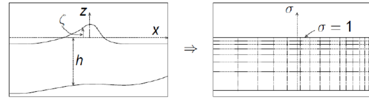
Figure 1: \sigma transformation
