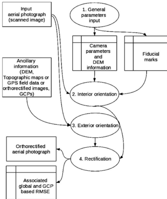
Fig. A2. General flow of the orthorectification procedure (Rocchini et al., 2012).
