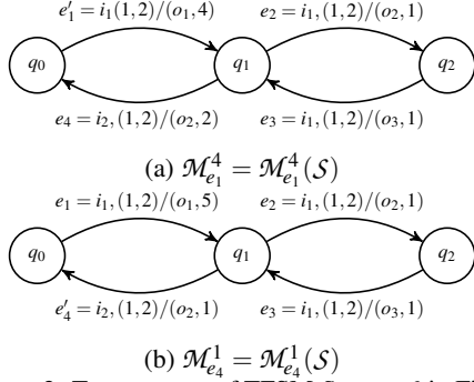
Figure 2: Two mutants of TFSM Spec = S in Fig. 1
