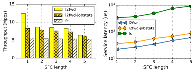
Fig. 4: The overhead of in-band data collection
