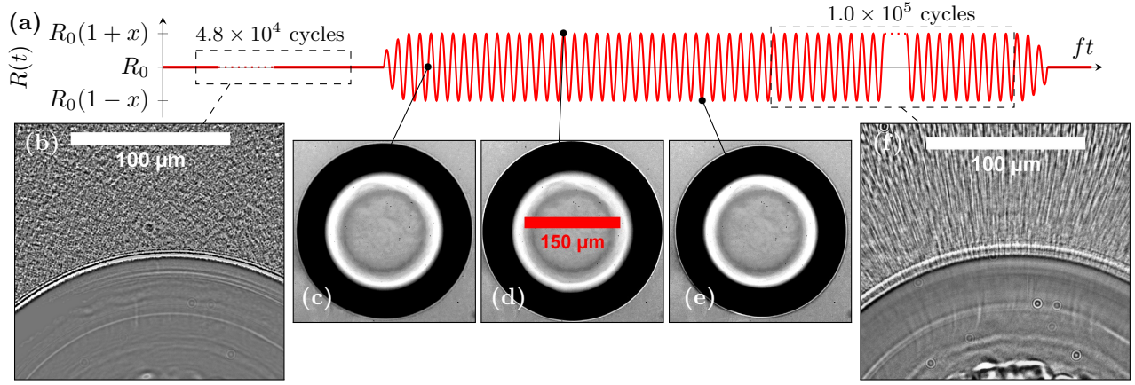
Fig. 6 Microstreaming around an ultrasound-driven pancake bubble, see SI Video 2. (a) Schematic representation of the bubble time series. (b) A bubble and its surroundings at rest, imaged using the real-time brightfield setup and averaged over N = 4.8 \times 10^4 cycles. The bubble is located at the bottom of the picture. (c-e) Instantaneous pictures of bubble oscillations acquired with the high-speed brightfield imaging setup, close to its radius at rest [Panel (c)], at its maximal radius [Panel (d)] and at its minimum radius [Panel (d)] for a bubble oscillation amplitude x = 0.03 . (f) Microstreaming observed when averaging brightfield images over N = 1.0 \times 10^5 cycles using the real-time setup .
