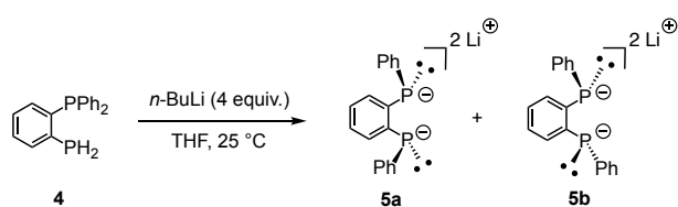
Scheme 1. Synthesis of dianions 5a,b from diphosphane 4 with excess n -BuLi.
