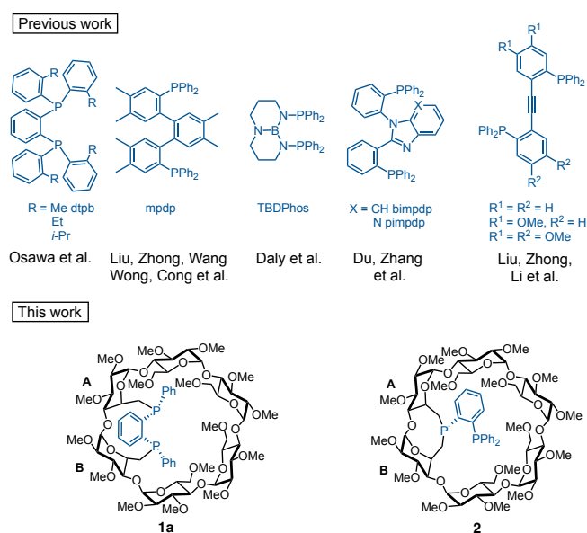
Figure 1. P,P ligands present in luminescent [CuX(PP)] complexes.
