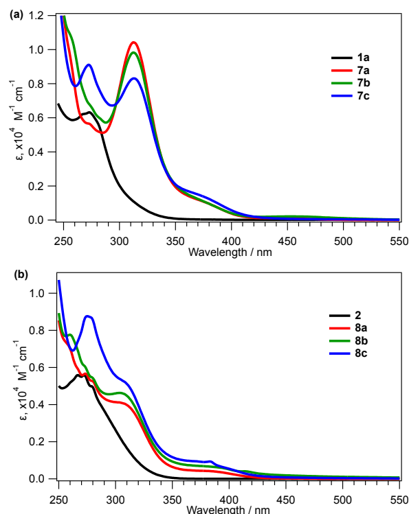
Figure 3. Absorption spectra of ligands 1a (a) and 2 (b) and their halide complexes 7a-c (a) and 8a-c (b) in \text{CH}_2\text{Cl}_2 .
