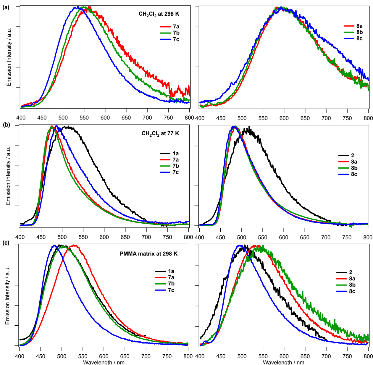
Figure 4. Emission spectra of ligand 1a and complexes 7a-c (column left), and ligand 2 and complexes 8a-c (column right) in (a) \text{CH}_2\text{Cl}_2 at 298 K; \lambda_{\text{ex}} = 380 \text{ nm} , (b) in \text{CH}_2\text{Cl}_2 at 77 K; \lambda_{\text{ex}} = 300 \text{ nm} for ligands and \lambda_{\text{ex}} = 380 \text{ nm} for complexes, (c) in PMMA 1 wt% at 298 K; \lambda_{\text{ex}} = 320 \text{ nm} for ligands and \lambda_{\text{ex}} = 380 \text{ nm} for complexes
