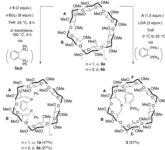
Scheme 2. Synthesis of diphosphanes 1 a , 2 and 3 a . [9]
