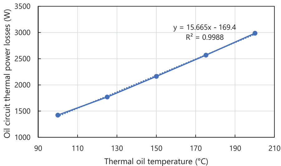
Figure 5. The thermal power losses in the oil circuit as a function of the oil temperature measured at the thermoacoustic engine inlet.
