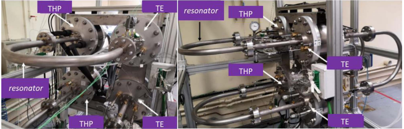
Figure 3. Pictures of the thermoacoustic WHRS.
