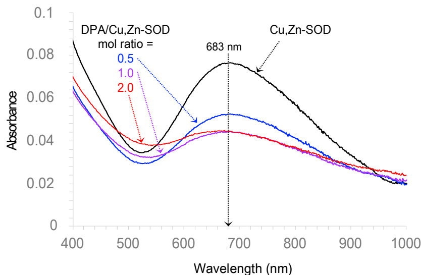
Figure 6. UV–visible spectrum of bovine erythrocyte Cu,Zn-SOD (10.14 mg/mL in phosphate buffer 100 \mu M, pH 7.4), either alone (black trace) or in the presence of DPA (0.5, 1.0, or 2.0 mol equivalent, blue, violet and red traces, respectively).
