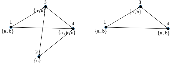
Fig. 2: On the left, an attributed graph \mathcal{G} = (V, E, A) , with V = \{1, 2, 3, 4\} , E = \{(1, 3), (4, 3), (1, 4), (3, 2), (2, 4)\} and A = \{a, b, c\} . On the right, the pattern (\{1, 3, 4\}, \{(1, 3), (3, 4), (1, 4)\}, \{a, b\}) .
