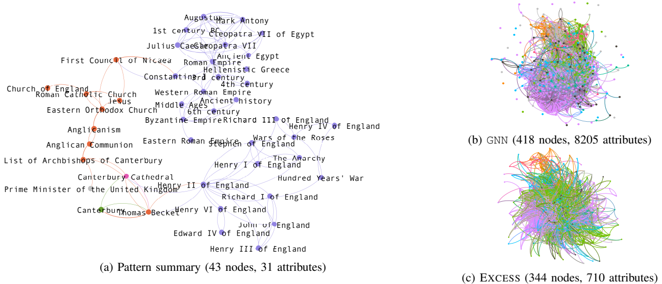
Fig. 5: A pattern summary (a) compared to its closest community or subgraph obtained with GNN (b) and EXCESS (c) methods. The colours of nodes and edges correspond to their respective categories in the Wikischools dataset.
