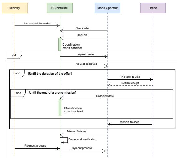
Fig. 3. Sequence diagram
