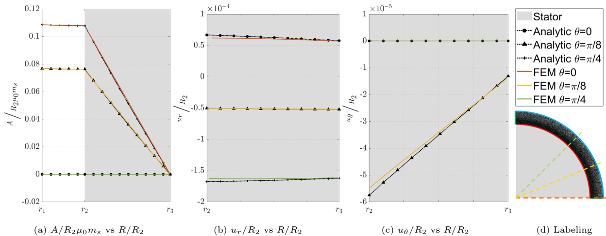
Figure 5: Difference between FEM (nonlinear magnetization response) and analytical predictions (linear magnetization response) for the cylindrical stator at large values magnetic field \|\mathbf{b}\| at three different angles. In (a) dimensionless magnetic potential A/R_2\mu_0m_s vs r , in (b) dimensionless radial displacement u_r/R_2 vs r and in (c) dimensionless tangential displacement u_\theta/R_2 vs r (dimensionless radius r = R/R_2 ).
