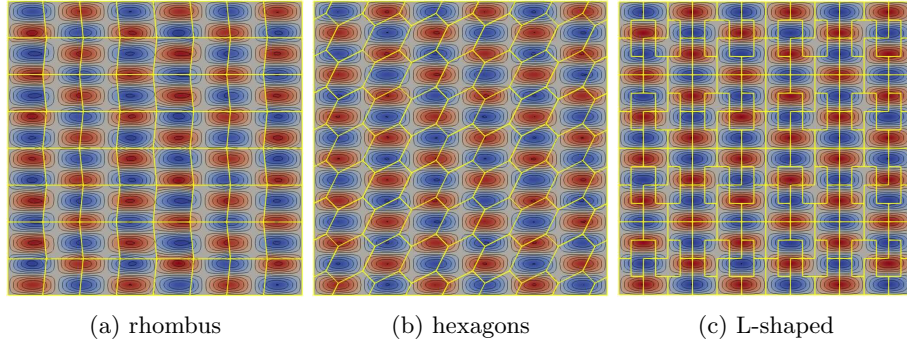
Fig. 3: Isolines of the solution using \mathcal{H} = H , \ell = 1 and k = 3 .
