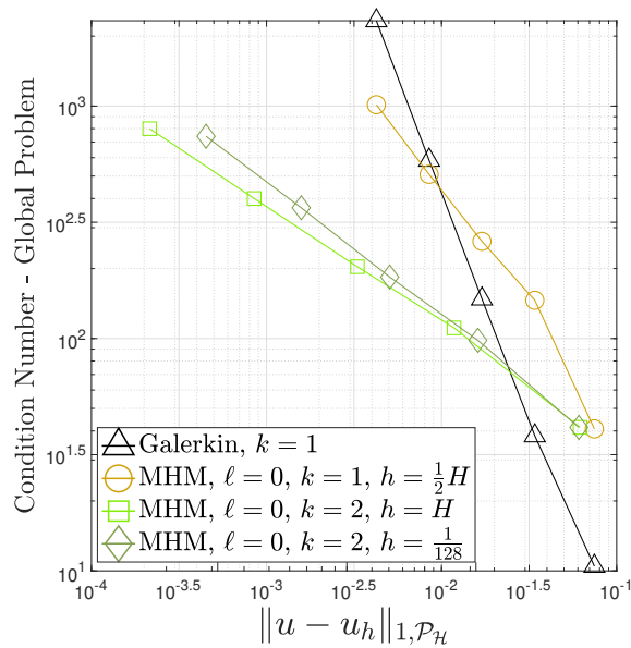
Figure 11: Error versus condition number of the matrix associated with the Galerkin method and the global problem matrix associated with the MHM method.
