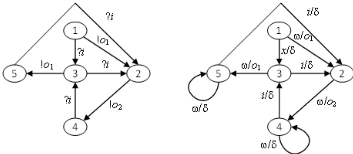
Figure 1: Automaton S and corresponding FSM M_S^{\delta\omega} .
