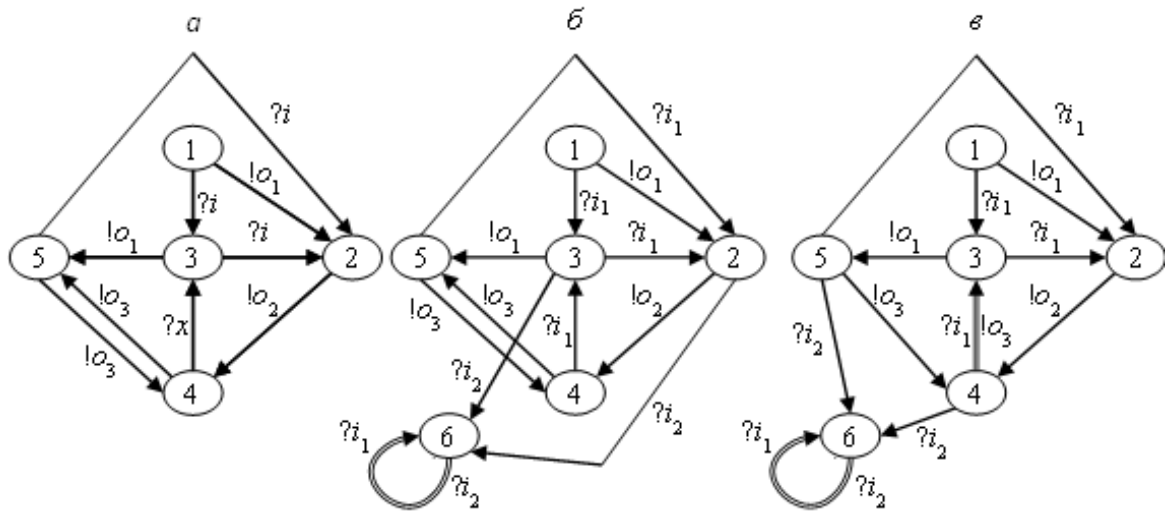
Figure 2: Automata with (stable) homing sequences.
