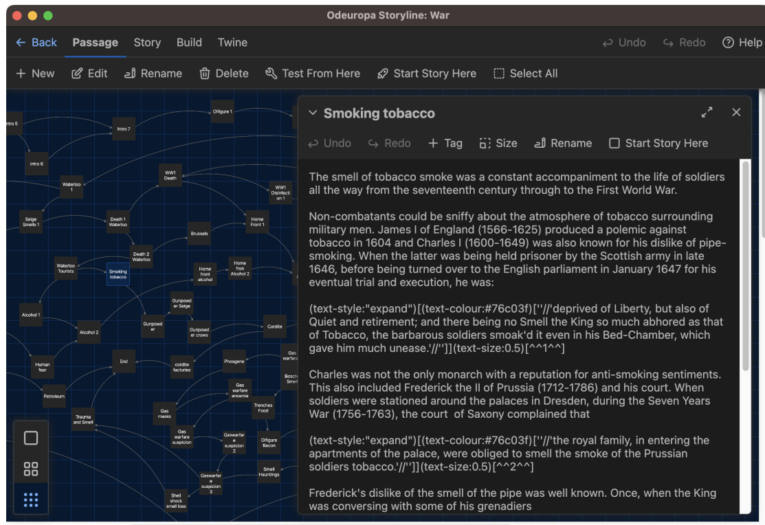
Figure 3: An example of story in Twine, with the story overview on the left and a story element in editing mode on the right. The connections between cards (the story elements) naturally give to the story a graph structure.
