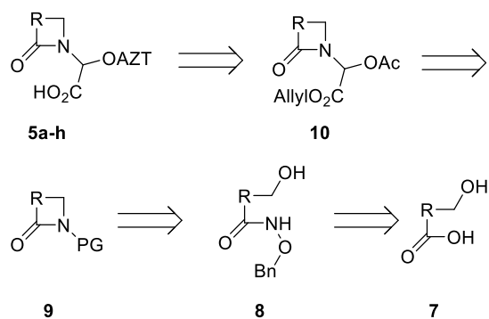
Scheme 3. Retrosynthetic analysis
