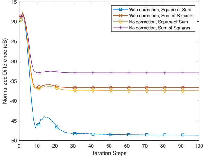
Fig. 1. MSE with or without correction.
