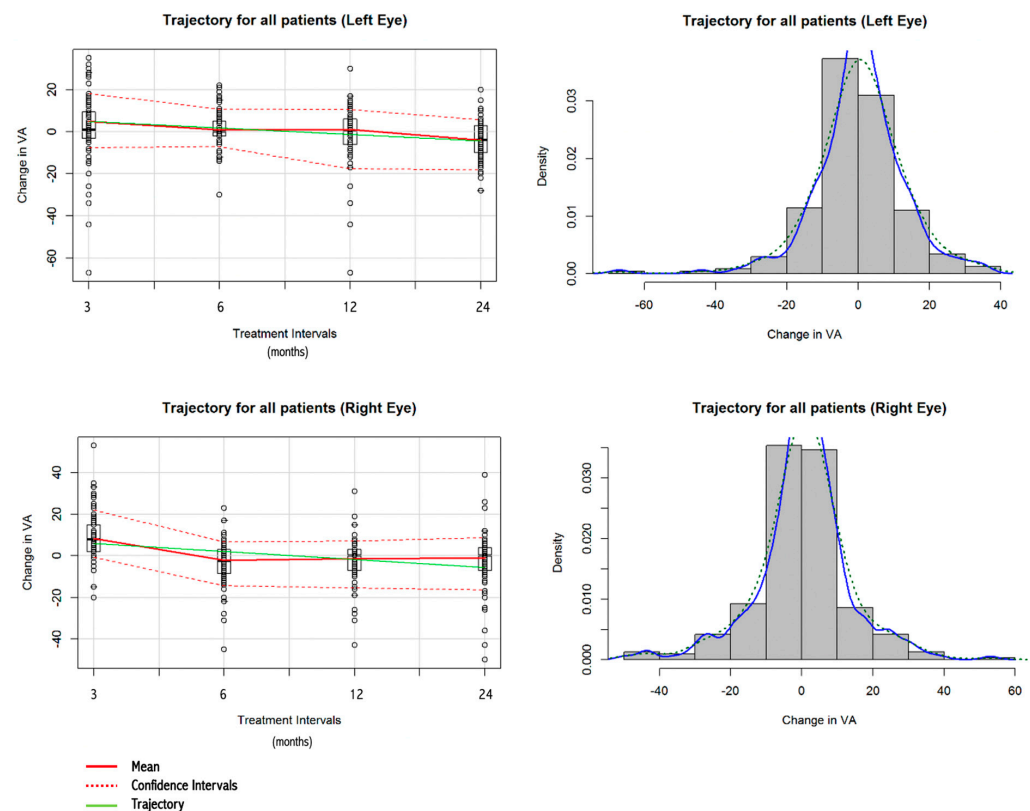
Figure 2. Distribution and trajectory plots to determine ceiling effects for all patients. The box plot with a curvature (left) demonstrates the trajectory of response for all patients collectively. There is a negative linear correlation. This suggests that, irrespective of response classification, all patients have a gradual decline in vision over time. The histogram (right) appears to be relatively normal overall, although closer inspection may suggest a very slight negative skew. A normal distribution would indicate no ceiling effect. The red line represents the mean (with confidence intervals), while the green line represents the trajectory. Blue lines illustrate the distribution.
