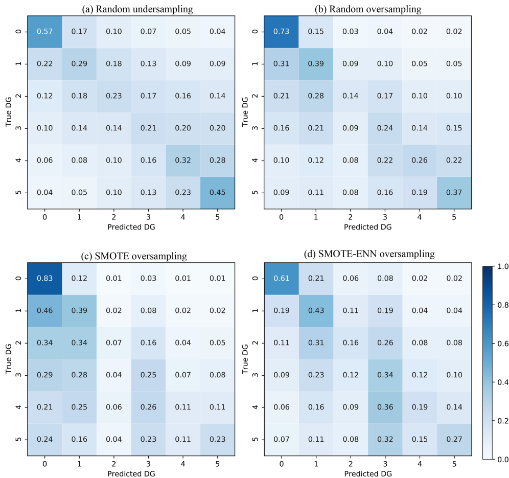
Figure 4. Confusion matrices for the four methods to solve the DG imbalance issue in DaDO. The values given in each main diagonal cell are the accuracy scores A_{DG} . All values are also represented by the colour scale.
