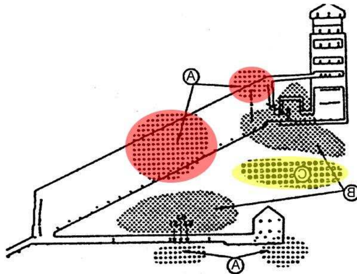
Microgravimetry survey - EDF Foundation - 1986
