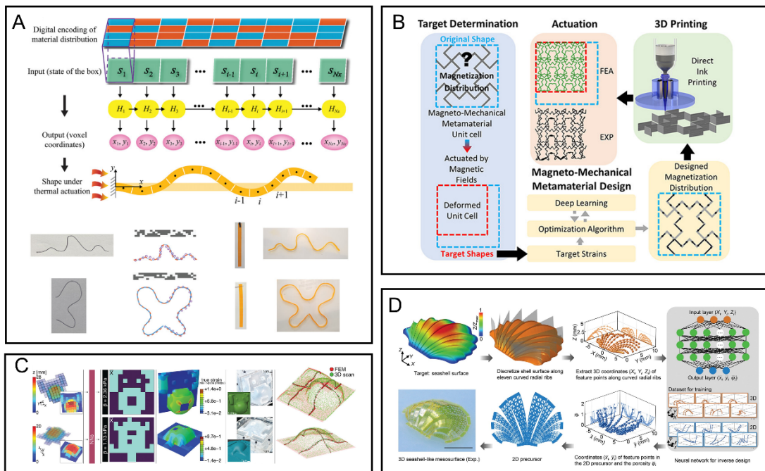
Figure 3. Applications of ML in various active material systems for designing active shape-change response. (A) Forward predictions using RNN-based ML and inverse design using
