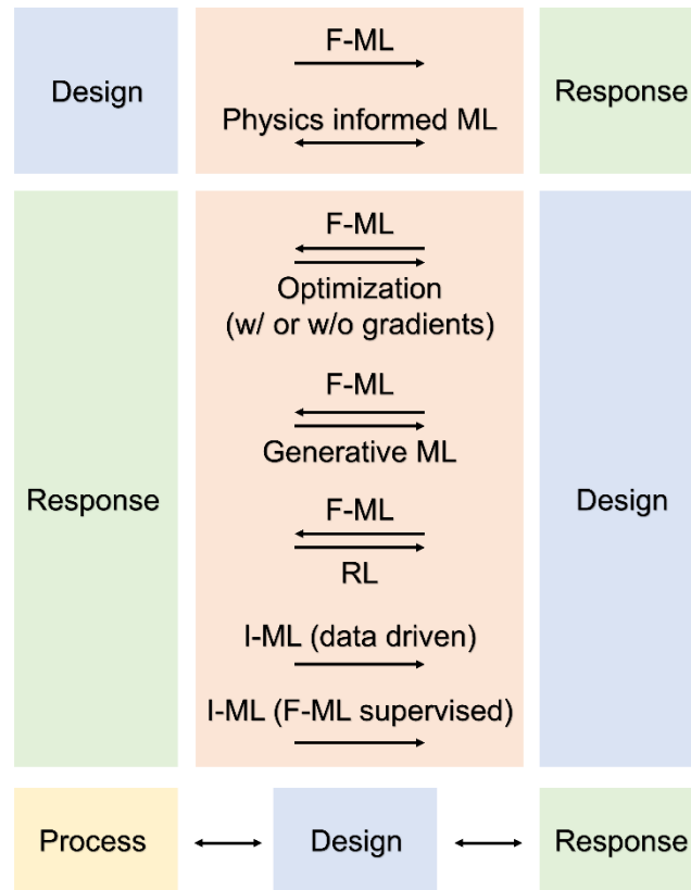
Figure 4. Overview of ML strategies for designs in 3D/4D printing.
