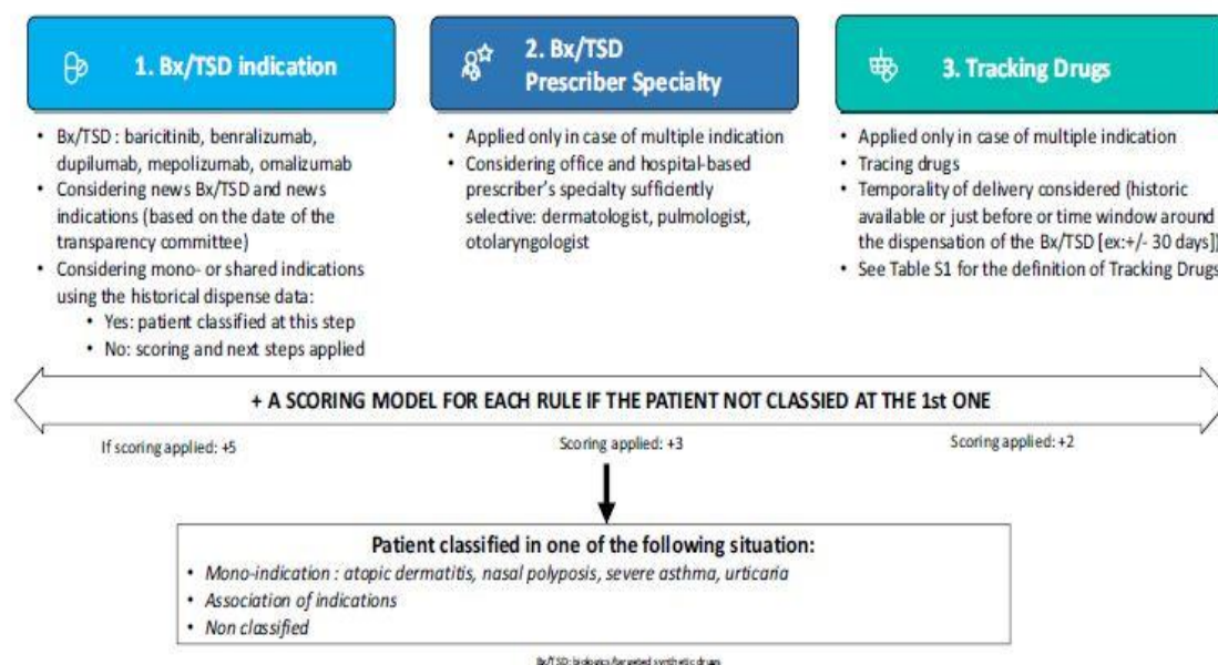
Figure 1 An algorithm constructed using consecutive steps including a scoring model and considering a maximum of 10-years historical dispense data.
