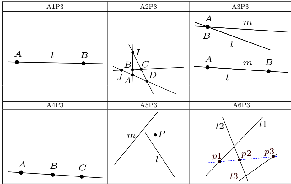
Fig. 1 Illustrations of the standard axiom system for projective space geometry
