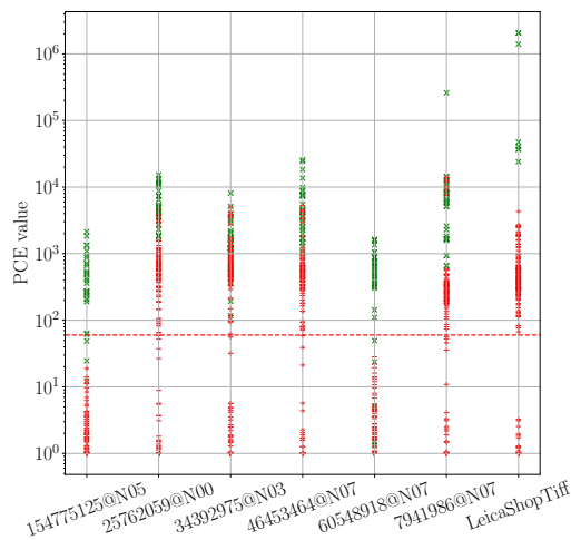
Figure 1: The original PCEs for the Leica Q2 camera and 7 different devices. The first 6 labels are the FlickrR identification names and the last one is images coming from a Q2 camera shared by the Leica Shop in Lille and developed using Adobe Lightroom in 8-bit Tiff format. Matching and mismatching tests are reported in green and red, respectively. The threshold of 60 is highlighted by the red dashed line.
