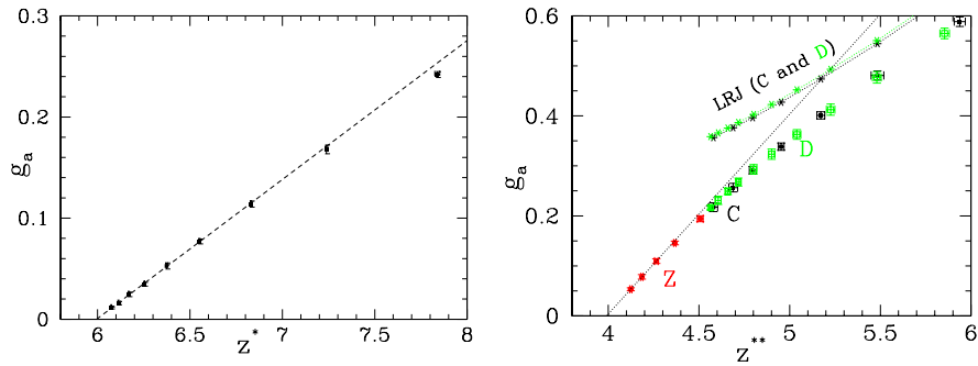
Fig. 14. Reduced shear moduli g_a versus corrected coordination number, in systems in isotropic compression. Left: frictionless case. Right: frictional case, with poorly coordinated states C and D, and state Z, assembled with infinite friction coefficient. z^{**} defined from z^* as in Eq. 34. Data points marked “LRJ”: prediction of the La Ragione-Jenkins scheme [65]. Dotted lines: linear fits.
