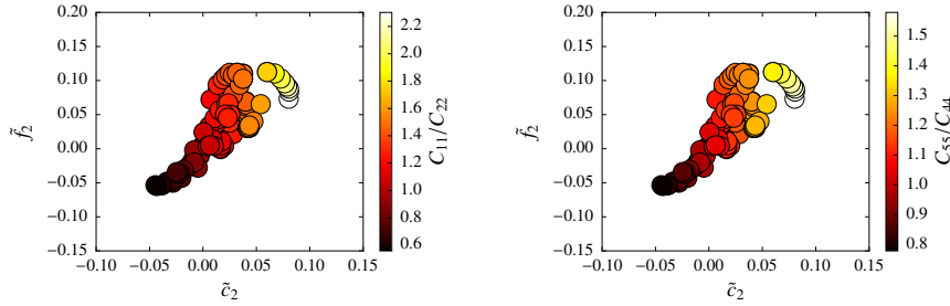
Fig. 17. Ratios of moduli characterizing elastic anisotropy: C_{11}/C_{22} (left) and C_{55}/C_{44} (right), with values encoded as colour intensity in \tilde{c}_2, \tilde{f}_2 plane.
