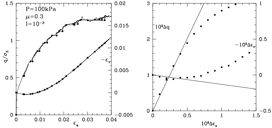
Fig. 25. Left: equilibration after small creep strain interval (beginning and end marked by round dots), followed by resumed strain rate-controlled loading. Right: deviatoric and volumetric strain curves, on small scale, upon resuming loading from equilibrated configurations. Straight lines: elastic response.
