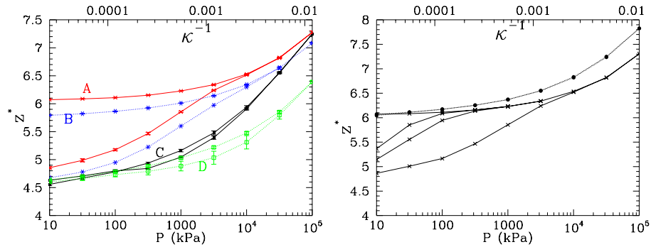
Fig. 6. Left: variations of rattler-corrected coordination number z^* in isotropic compression cycle for states A to D. Right: effects on z^* of smaller pressure cycles in A systems, with load reversals at 316.2 kPa, 3.162 MPa and 31.62 MPa, instead of 100 MPa.
