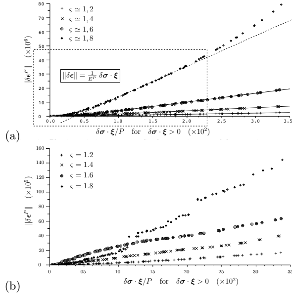
Fig. 29. \|\delta\boldsymbol{\varepsilon}^P\| versus [\boldsymbol{\xi} \cdot \delta\boldsymbol{\sigma}]_+ , for different stress ratios \zeta and \kappa = 10^4 . (a): type I strains. (b): type II strains.
