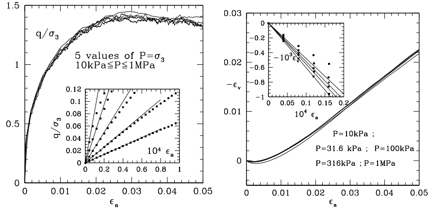
Fig. 23. Normalized deviator q/\sigma_3 (left) and volumetric strain -\varepsilon_v versus axial strain \varepsilon_a (right) in triaxial compression of C-type system with different values of initial isotropic pressure P = \sigma_3 . Insets show very small strain range, with straight line slopes equal to elastic prediction.
