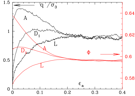
Fig. 9. Deviator stress q and solid fraction \Phi versus axial strain \varepsilon_a in simulated triaxial tests ( P_0 = 100 kPa or \kappa \simeq 8000 ) carried out with initial states A, D and L.
