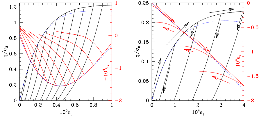
Fig. 24. Behaviour of dense systems upon load reversal (reversing of the sign of \varepsilon_a ) at different stages within initial regime of type I strain in triaxial compression at constant lateral stress 100 kPa. Left: high coordination number (A). Right: low coordination number (C). Thin dotted lines: response on ignoring the creation of new contacts.
