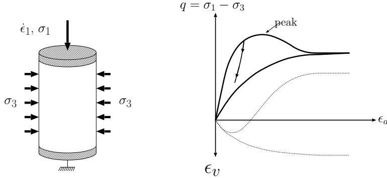
Fig. 8. Left: Schematic view of triaxial compression test. Right: Aspect of deviatoric stress q (solid line) and volumetric strain \varepsilon_v (thin dotted line) versus axial strain \varepsilon_a = \varepsilon_1 for initially dense (upper curves for both q and -\varepsilon_v ) and loose (lower curves) states.
