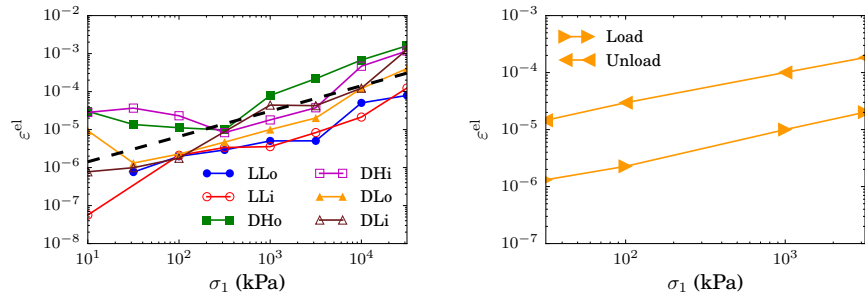
Fig. 20. Left: quasielastic range near equilibrated state along compression path of samples of different types, versus axial stress \sigma_1 . Straight line has slope 2/3. Right: elastic domain in loading and unloading in states DLo.
