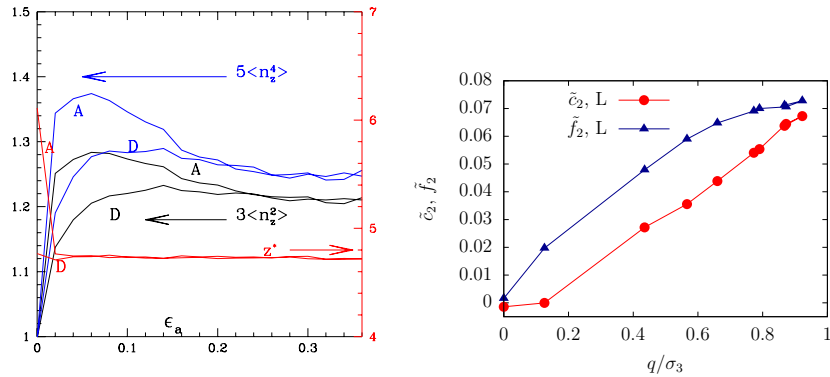
Fig. 10. Left: evolution of coordination number z^* and fabric parameters (here n_z = n_1 ) in dense and medium dense systems A and D in triaxial compression test, versus \varepsilon_a . Right: increase of anisotropy parameters \tilde{c}_2 and \tilde{f}_2 (see Eqns. 16 and 19) in loose system L, versus normalized deviator q/\sigma_3 .
