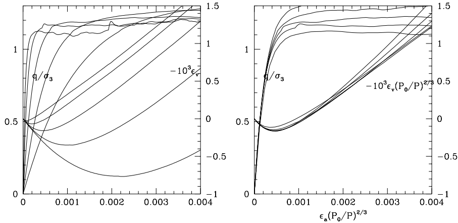
Fig. 22. Normalized deviator q/\sigma_3 and volumetric strain -\varepsilon_v versus axial strain \varepsilon_a in triaxial compression of A-type system with different values of initial isotropic pressure P = \sigma_3 , from 10 kPa ( \kappa \simeq 39000 ) to 1 MPa ( \kappa \simeq 1800 ). Left: natural strains; right: rescaled strains, using P_0 = 100 kPa.
