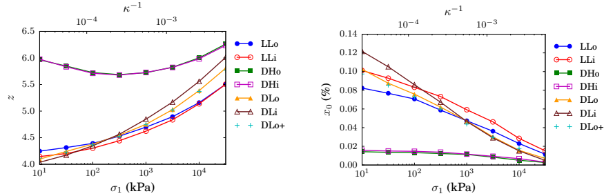
Fig. 1. Coordination number z (left graph) and rattler fraction x_0 (right graph) versus axial stress \sigma_1 , or \kappa^{-1} , in oedometric compression of the different initial states (“DLo+” data pertain to DLo-type sample with 13500 grains instead of 4000, showing size independence).
