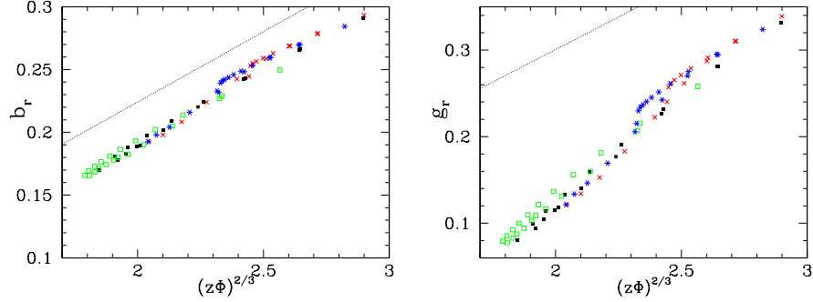
Fig. 12. Left: reduced bulk modulus b_r = B/(\tilde{E}^{2/3}P^{1/3}) , for systems A to D in compression cycle, versus (z\Phi)^{2/3} . Right: same graph for reduced shear modulus g_r = G/(\tilde{E}^{2/3}P^{1/3}) . Dotted lines show Voigt predictions.
