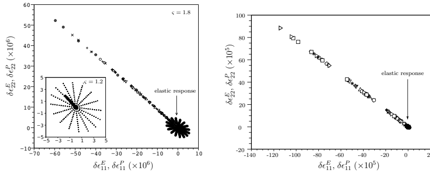
Fig. 28. Decomposition of strain increments into elastic and plastic parts. Left: stress probes in type I strain regime with \zeta = 1.8 (main plot) or \zeta = 1.2 (inset). Right: stress probes in type II strain regime ( \zeta = 1.8 ).
