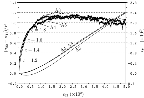
Fig. 26. Biaxial test on dense sample with low coordination number, for different stiffness number \kappa : 10^5 , 10^4 and 10^3 . Written values of \zeta correspond to chosen investigation points.
