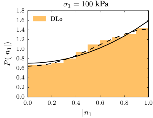
Fig. 2. Anisotropy of contact orientations: histogram of |n_1| values in system DLo at \sigma_1 = 100 kPa, and its representation with expansion (14), truncated after order 2 (solid line) or order 4 (dashed line).
