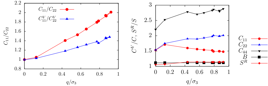
Fig. 21. Left: ratio of longitudinal moduli versus normalized deviator q/\sigma_3 in triaxial compression of loose systems (L), along with Voigt prediction. Right: ratios of Voigt predictions to measured moduli, and ratio S_P^R/S_P , versus q/\sigma_3 .
