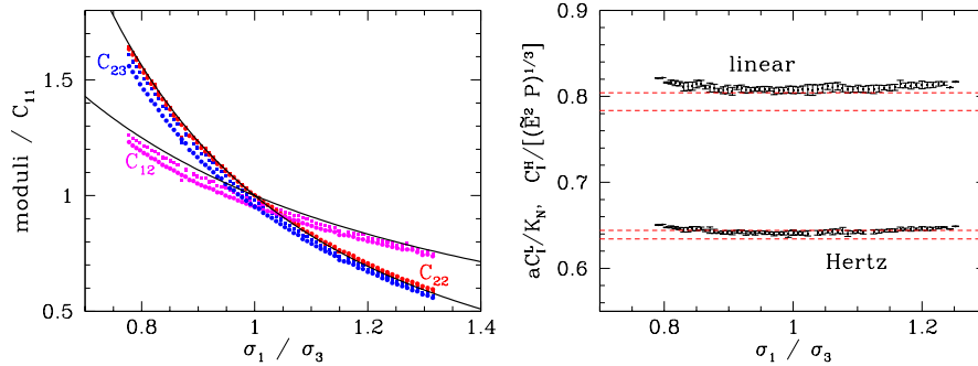
Fig. 15. Elastic moduli of nearly rigid frictionless bead packs under triaxial compression ( \sigma_1 \geq \sigma_2 = \sigma_3 ) or extension ( \sigma_1 \leq \sigma_2 = \sigma_3 ). Left: ratio of moduli to C_{11} , for Hertzian (square dots) or linear (round dots) contact elasticity. Continuous lines: behaviour predicted in Eqs. 36. Right: dominant eigenvalue C_I (data points) of tensor of elastic moduli, compared to Reuss prediction (between dashed lines) with Hertzian ( C_I^H ) or linear ( C_I^L ) contact elasticity.
