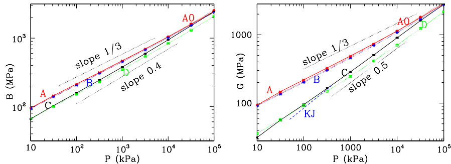
Fig. 11. Bulk (left) and shear (right) moduli versus confining pressure on doubly logarithmic scale in isotropic compression of states A, B, C, D. Line marked “KJ”: fit through experimental data of Ref. [9].
