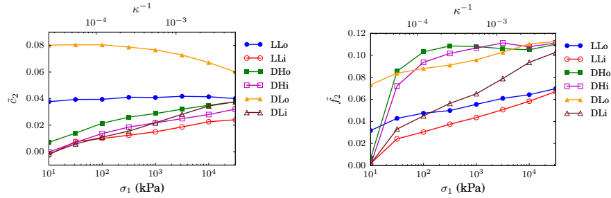
Fig. 3. Fabric anisotropy parameter \tilde{c}_2 and force anisotropy parameter \tilde{f}_2 versus axial stress \sigma_1 or \kappa^{-1} in oedometric compression of the different initial states.
