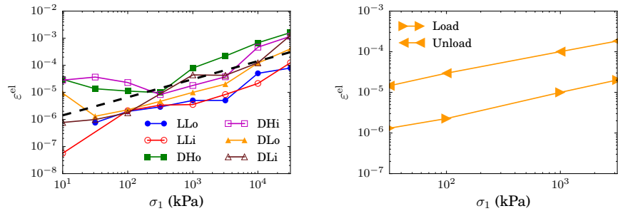
Fig. 20. Left: quasielastic range near equilibrated state along compression path of samples of different types, versus axial stress \sigma_1 . Straight line has slope 2/3 . Right: elastic domain in loading and unloading in states DLo.
