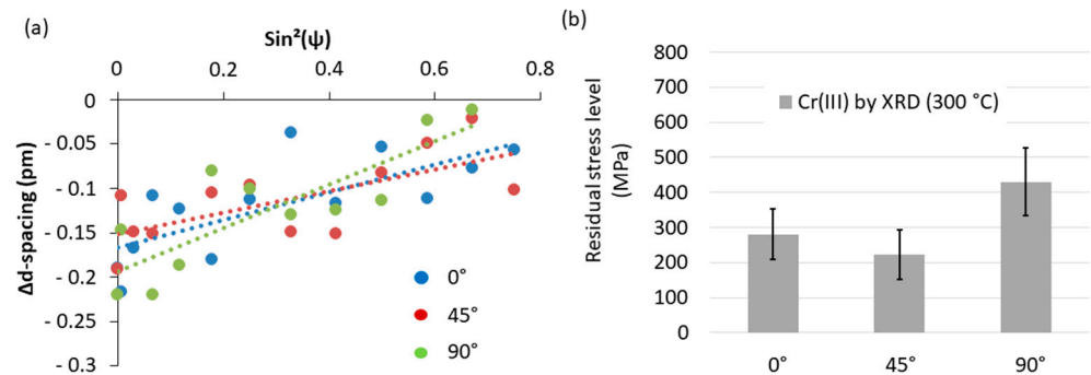
Figure 7. (a) Evolution of the \Delta d spacing as a function of \sin^2 \psi for the plane (211). A total of 0°, 45°, and 90° stands for the three different values of \varphi . (b) Results of the XRD residual stress level measurements on crystallized trivalent chromium.
