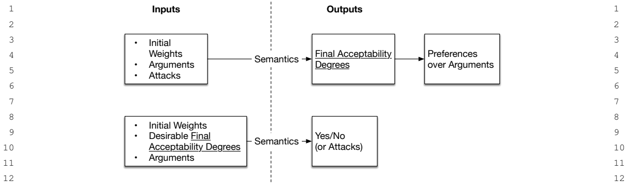
Fig. 1. The process (top) by which a gradual semantics is applied to compute an acceptability preference between arguments and (bottom) the inverse problem considered in this paper. The “final acceptability degrees” are now used as input. That is, given arguments, initial weights, and desirable final acceptability degrees, can we find a suitable set of attacks?
