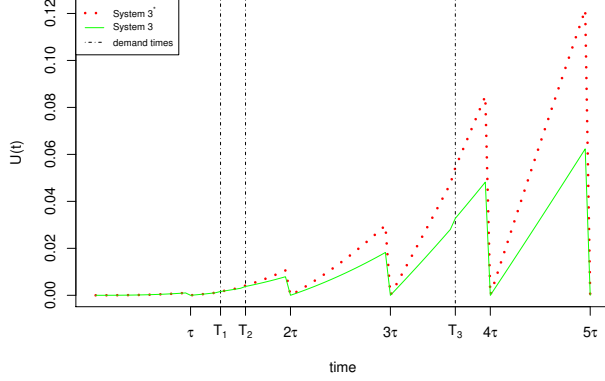
Figure 8: Time dependent Unavailability for different demand situations
