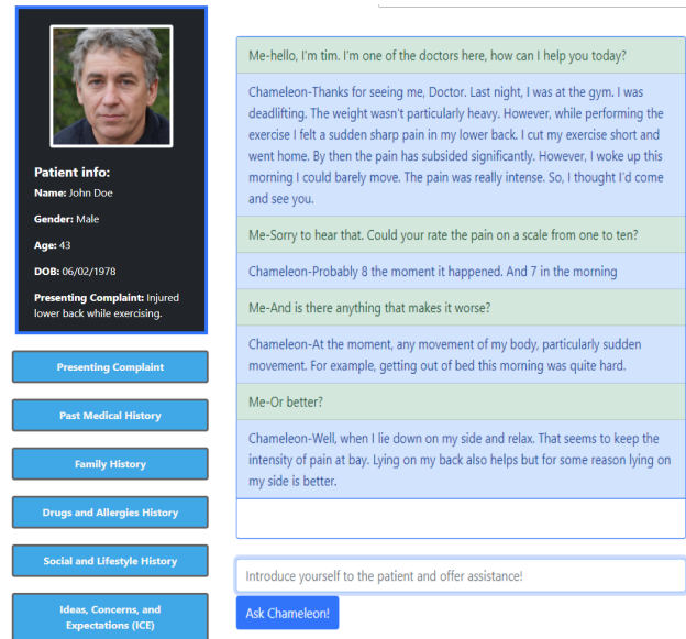
Figure 2: Screenshot of the Chameleon online interface.
