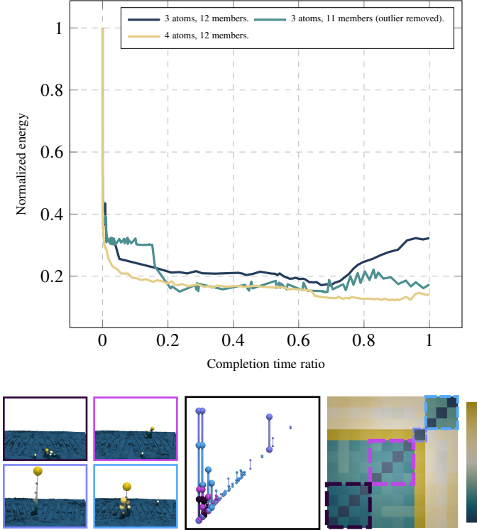
Fig. 17. Evolution of the (normalized) energy E_D along the optimization (top curves), with our multi-scale strategy, for the Volcanic eruption ensemble , for distinct initializations. The ground-truth classification of this ensemble contains 3 classes [79], including one outlier (light purple entry in the bottom views, from left to right: terrain view of the data, aggregated birth/death space, distance matrix). A clear energy increase can be observed when considering the entire ensemble (black curve), while a more characteristic oscillating behavior occurs when discarding the outlier (green curve). When initializing the optimization with 4 atoms (1 per class, plus 1 for the outlier), the optimization results in few oscillations and a consistent energy decrease (yellow curve).
