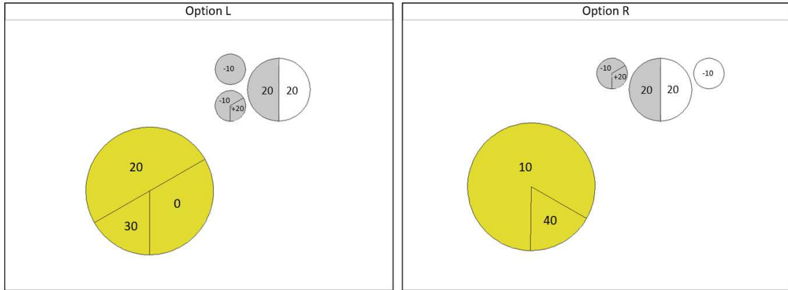
Figure 8: Image example 2
