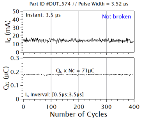
Fig. 3. The gate current ( I_G ) remains nearly constant between @Cycle1 and @Cycle400. Gate charge ( Q_G ) about the same 71 \mu C for 400 cycles.
