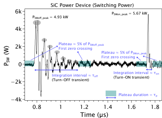
Fig. 4. Instantaneous switching power of a SiC device. The criteria used to define the new integration intervals define a plateau. Parameters: \tau_{off} = 400 \text{ ns} , \tau_{on} = 40 \text{ ns} , and \tau_p = 40 \text{ ns} (adjustable). The number of positive areas (gray ellipses) is also a reference.
