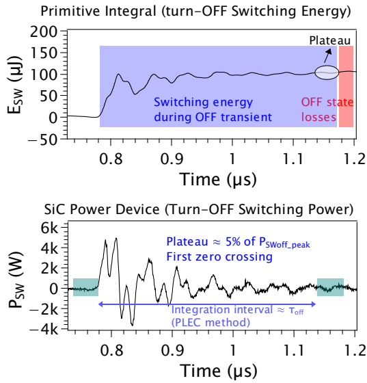
Fig. 5. Primitive integral of switching power during turn-OFF event. Parameters: \tau_{off} = 400\text{ ns} .
