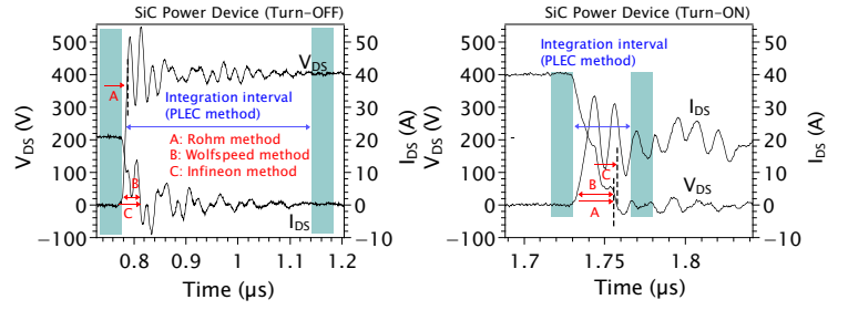
Fig. 7. Waveforms of drain-source voltage and drain-source current during turn-OFF and turn-ON events. Red arrows correspond to the integration limits for the methods A and B, and the final integration limit for the method C.
