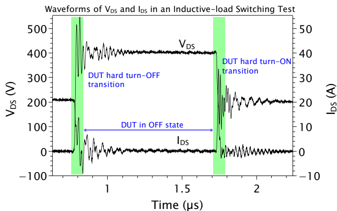
Fig. 3. Waveforms of drain-source voltage and drain-source current in an inductive-load switching test. Green areas highlight the switching transient fronts.
