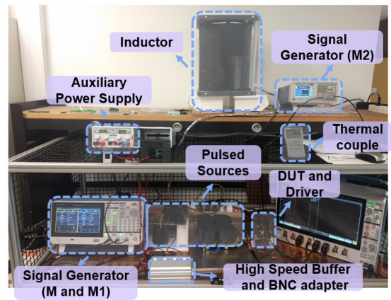
Fig. 2. DST bench used for switching characterization.
