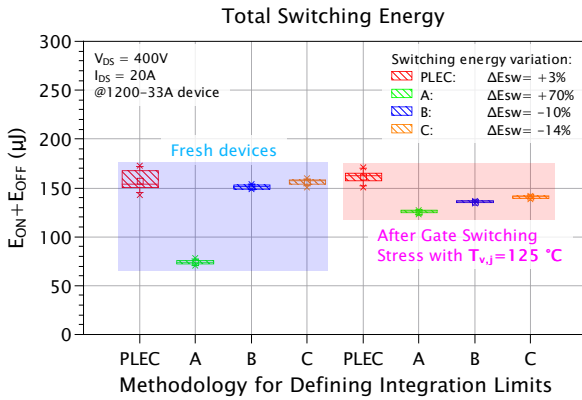
Fig. 11. Total switching energy according to PLEC, A, B and C methods. GSS test is performed with devices under 125 °C.
