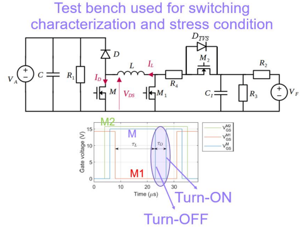
Fig. 1. Electrical schematic of double source test.
