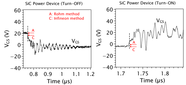
Fig. 8. Waveforms of gate-source voltage during turn-OFF and turn-ON events. The red arrows correspond to the initial integration limit for the method A and C.
