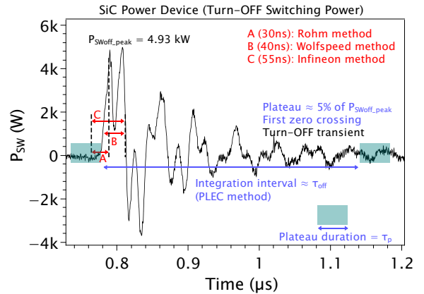
Fig. 9. Switching power during turn-OFF event. The red arrows correspond to the integration limits for the methods A, B, and C. The blue arrows correspond to PLEC method. Parameters: \tau_{off} = 400\text{ ns} , and \tau_p = 40\text{ ns} (adjustable).
