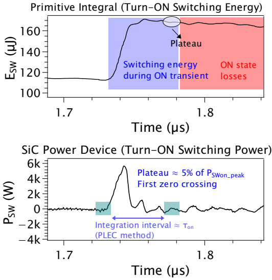
Fig. 6. Primitive integral of switching power during turn-ON event. Parameters: \tau_{on} = 40\text{ ns} .
