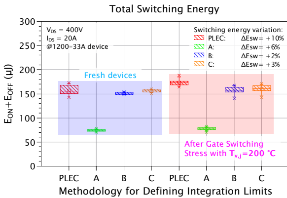
Fig. 12. Total switching energy according to PLEC, A, B and C methods. GSS test is performed with devices under 200 °C.
