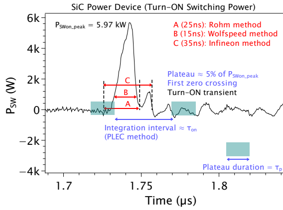
Fig. 10. Switching power during turn-ON event. The red arrows correspond to the integration limits for the methods A, B, and C. The blue arrows correspond to PLEC method. Parameters: \tau_{on} = 40 ns , and \tau_p = 40 ns (adjustable).
