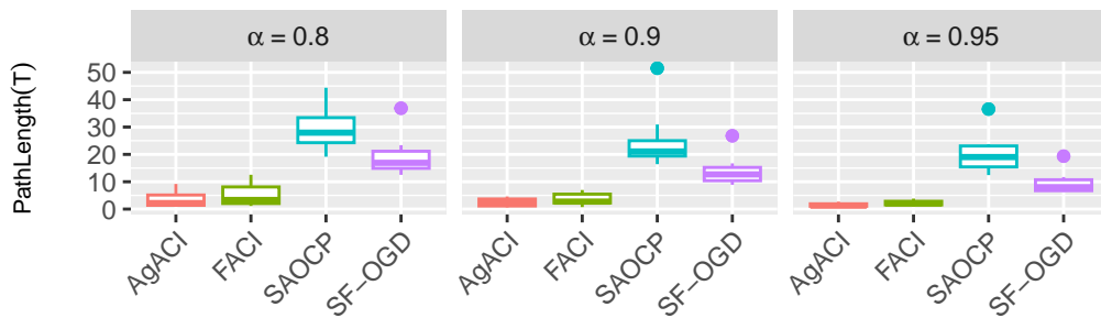
Figure 10: Coverage errors, mean interval widths, and path lengths of prediction intervals generated with each ACI method based on forecasts from each of the 19 underlying influenza forecasting models.
