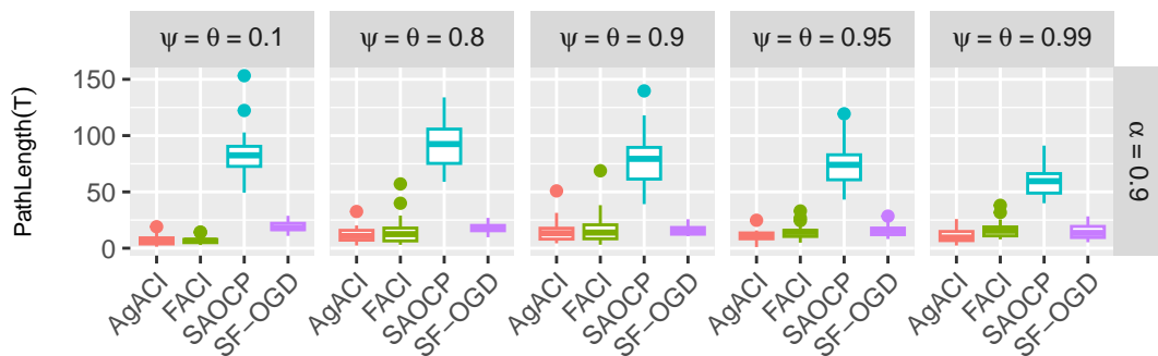
Figure 6: Coverage errors, mean interval widths, and path lengths for the first simulation study with target coverage \alpha = 0.9 .
