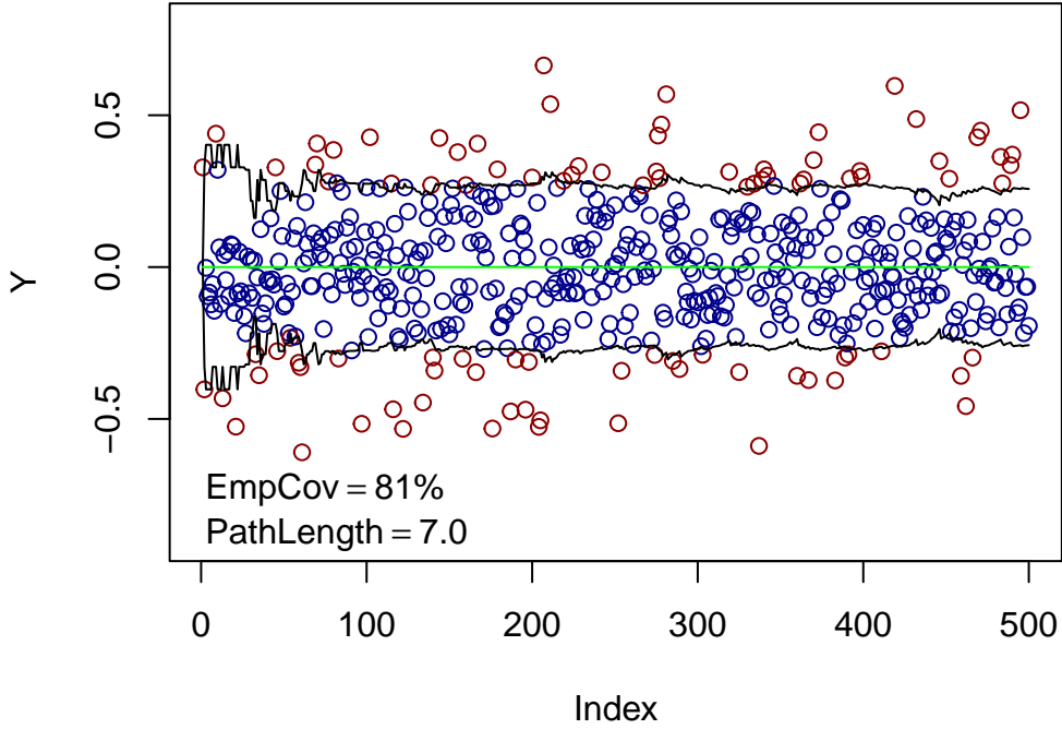
Figure 3: Example 80% prediction intervals generated by the FACI algorithm with starting values \theta_1 = 0.8 . Blue and red points are observations that fell inside and outside the prediction intervals, respectively.
