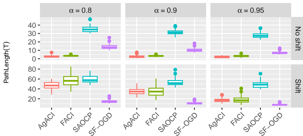
Figure 14: Coverage error, mean interval width, and path length for \alpha = 0.8, 0.9, 0.95 and simulations with and without distributional shift.
