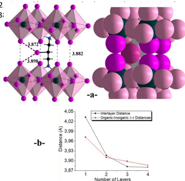
Fig. 2 a) Partial view of the structure of (DicI)(MA) 2 Pb 3 I 10 showing the I (ap) ...I (ap) and I (ap) ...I (orga) interactions (I (ap) : apical iodide of perovskite layers; I (orga) : iodine of DicI 2+ ; distances in Å) at the organic-inorganic interface: ball and stick (left) and space-filling (I radius of 1.98 Å, right) representations; b) d(I (ap) ...I (ap) ) and d(I (ap) ...I (orga) ) = f(n) in (DicI)(MA) n-1 Pb n I 3n+1 (n = 1-4).
