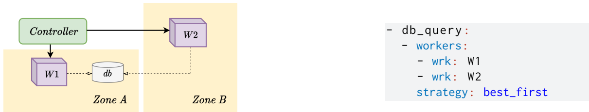
Figure 1: Example of function-execution scheduling problem and APP script.
