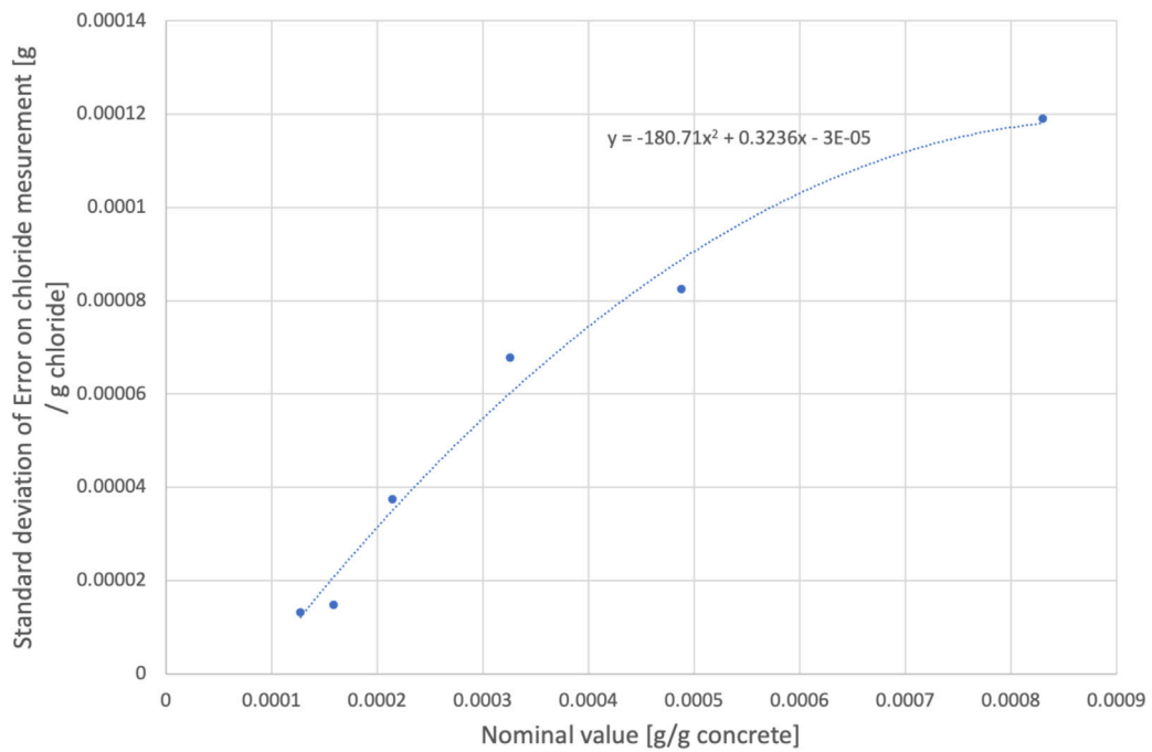
FIGURE 6 Evolution of the standard deviation of error of measurement as a function of reference.
