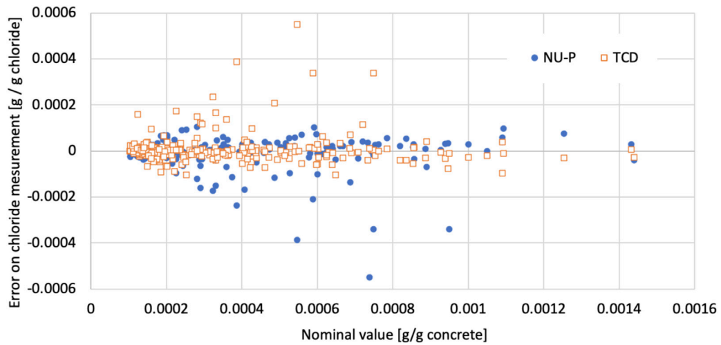
FIGURE 5 Plot of the error of measurement as a function of the nominal content for the two laboratories (NU-P and TCD).
