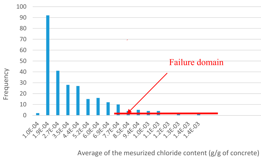
FIGURE 8 Presentation of the failure zone for average chloride contents.
