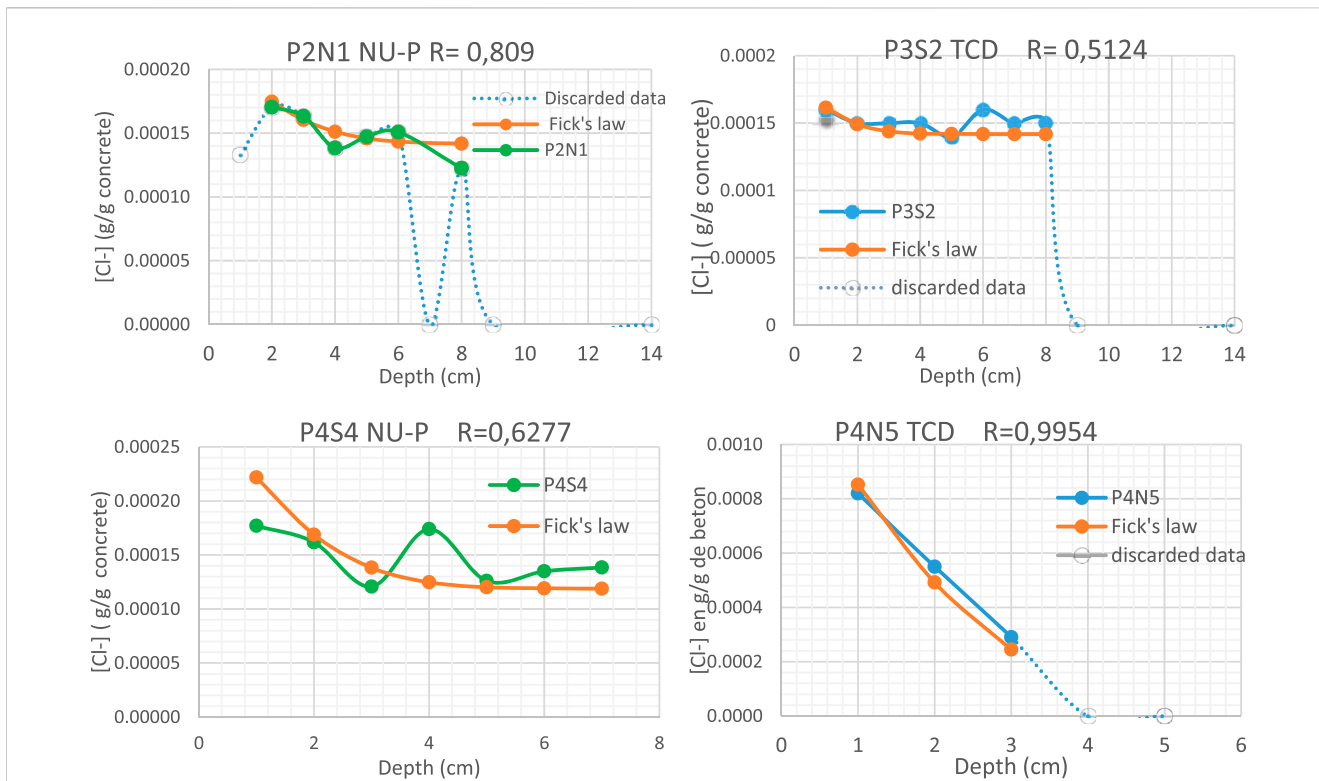
FIGURE 4 Examples of profiles obtained in three beams (P2, P3, and P4), on north and south faces (N/S) for two operators (TCD and NU) with a few outliers excluded from the analysis (discarded data) and discarded profiles.
