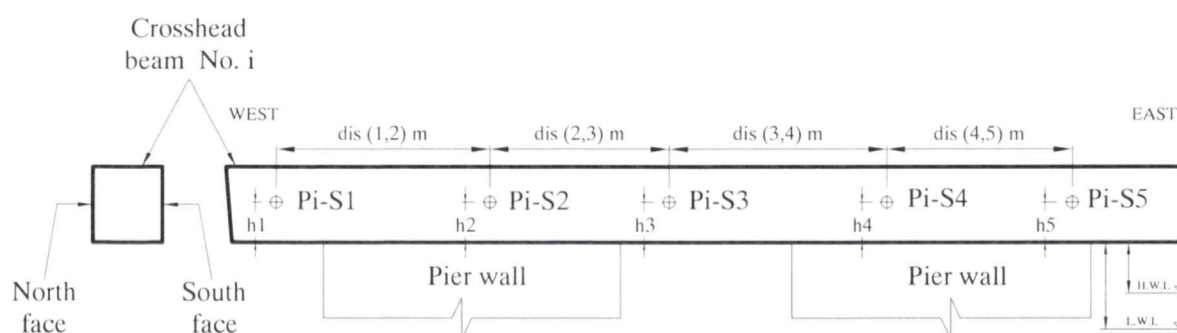
FIGURE 2 Cores symbolizing system (Kenshel, 2009, pp. 117).
