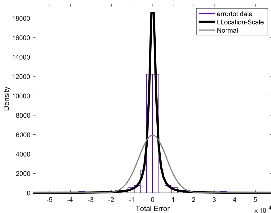
FIGURE 7 Normal and t-location scale pdf used for fitting the distribution of errors.
